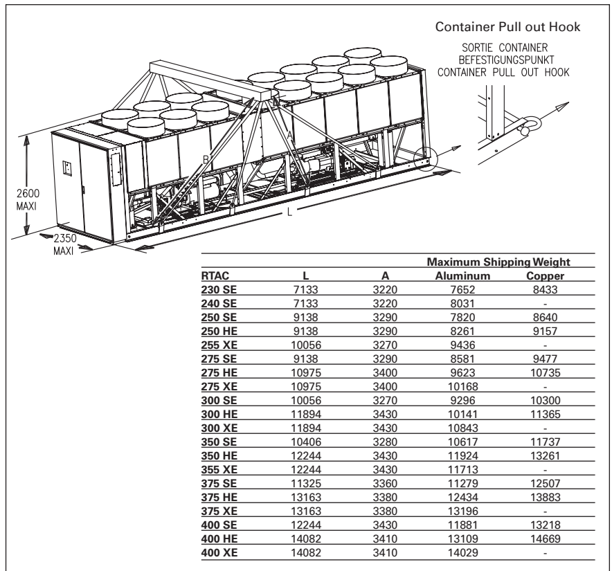
Figure 4 – Rigging the Unit, Sizes 230-400
