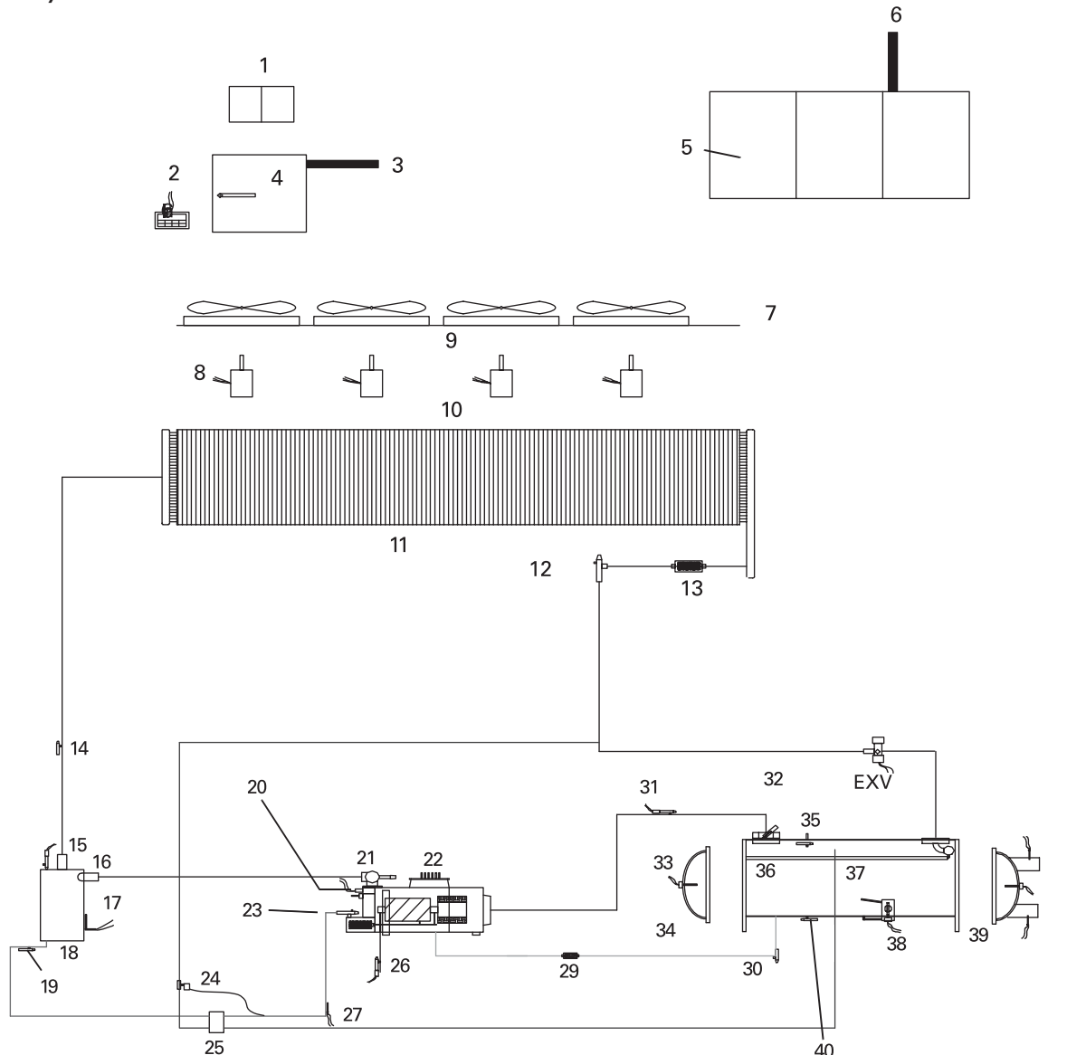
Figure 7 – System Schematic
